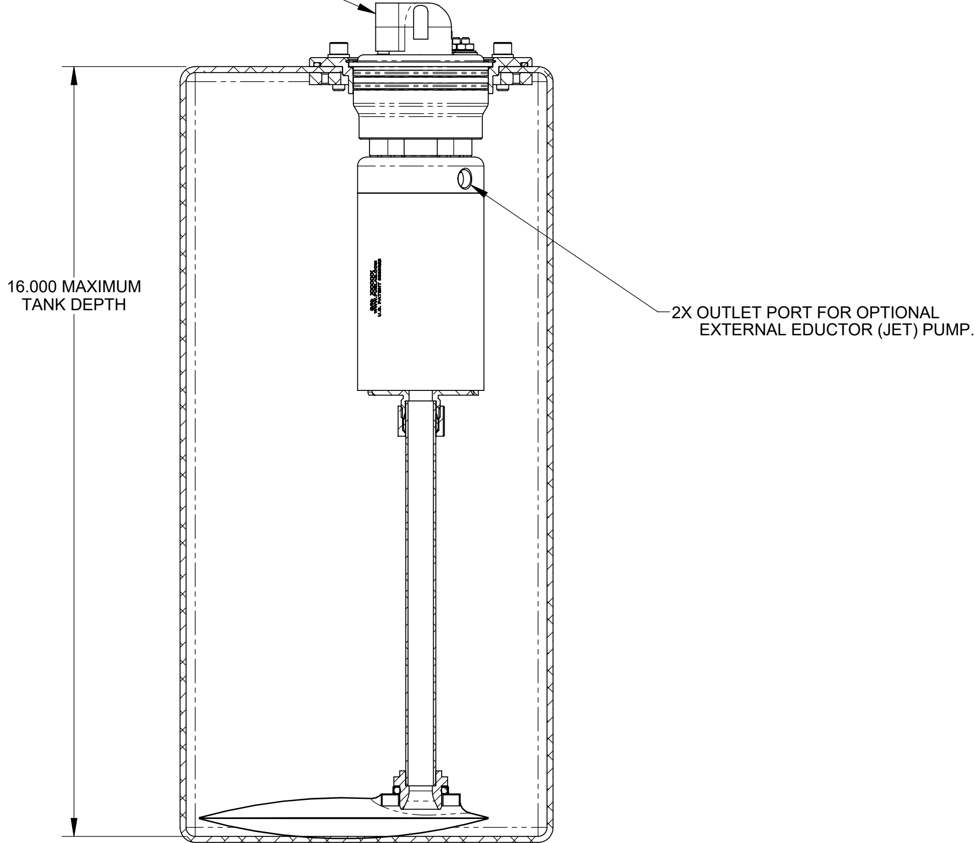
SECTION A-A MAXIMUM INSTALLATION HEIGHT WITH MODELS 90902, 91901 AND 92902 SHOWN ABOVE SCALE: 1/2
