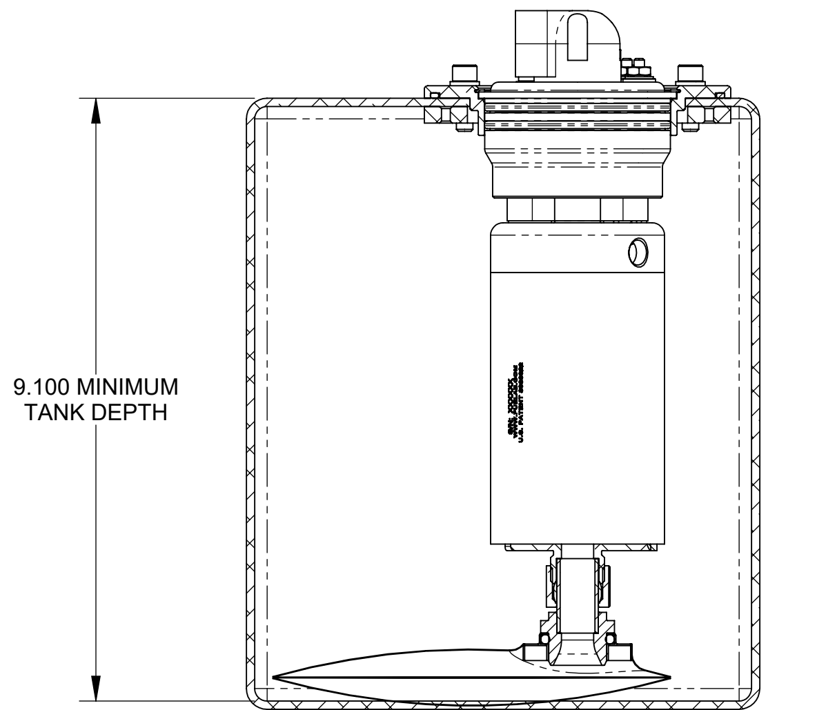
SECTION A-A MINIMUM INSTALLATION HEIGHT WITH MODELS 90902, 91901 AND 92902 SHOWN ABOVE SCALE: 1/2
